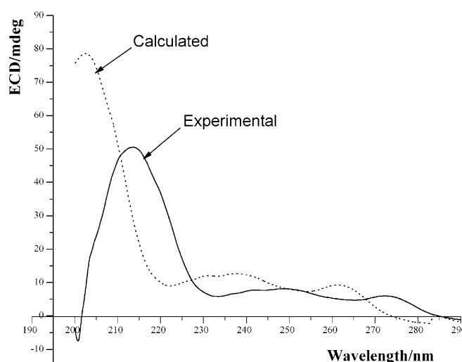
Figure 4. The theoretical simulated ECD spectrum (dotted trace) for the R -configuration of compound 4f by the means of the TD-DFT/B3LYP/6-31 + G* method, compared to the experimental spectrum (full trace).
