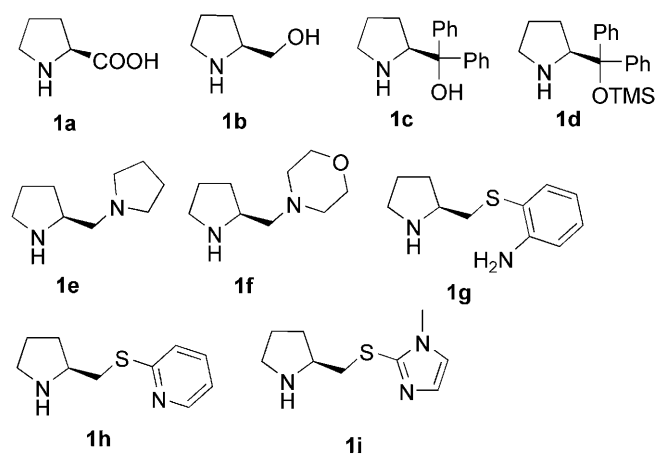
Figure 3. Screened organocatalysts.
