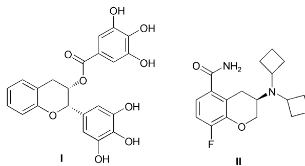
Figure 1. Some representative examples of biologically active compounds derived from 3-nitro-2 H -chromenes.
