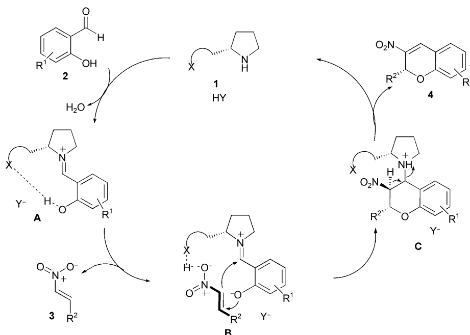
Figure 2. proposed mechanism of aromatic iminium activation for the organocatalyzed asymmetric tandem oxa-Michael–Henry reaction.
