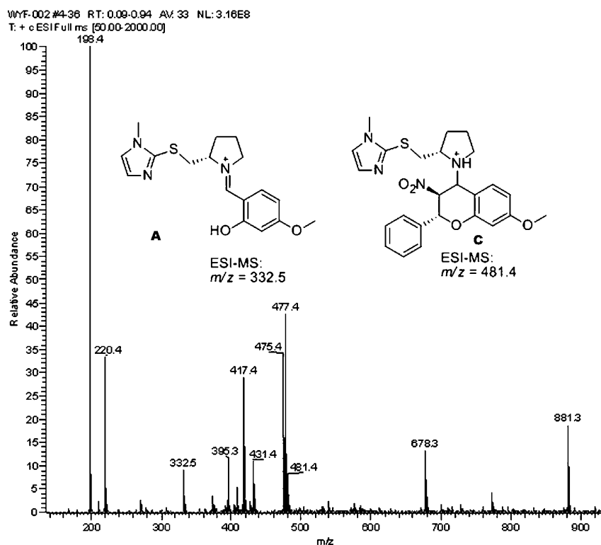
Figure 5. ESI-mass spectra: the existence of intermediates A and C in the reaction mixture was confirmed.
