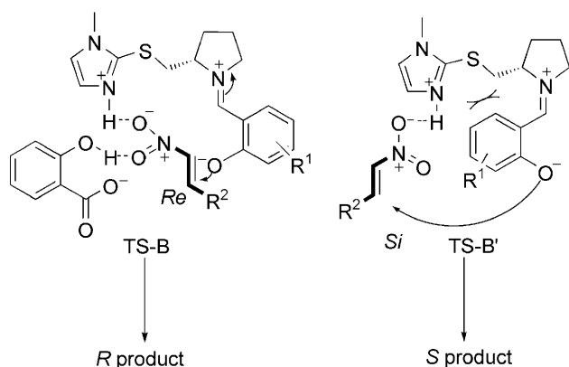
Figure 6. The proposed transition states in the tandem oxa-Michael–Henry reaction.
